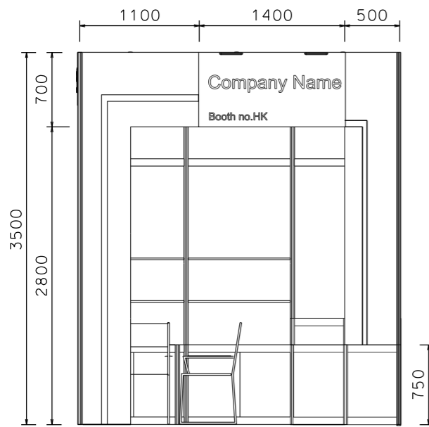
FRONT ELEVATION
