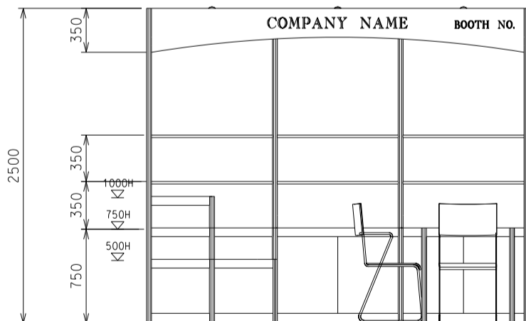
ELEVATION 3M(W) X 3M(D) X 2.5M(H) Standard Booth B
